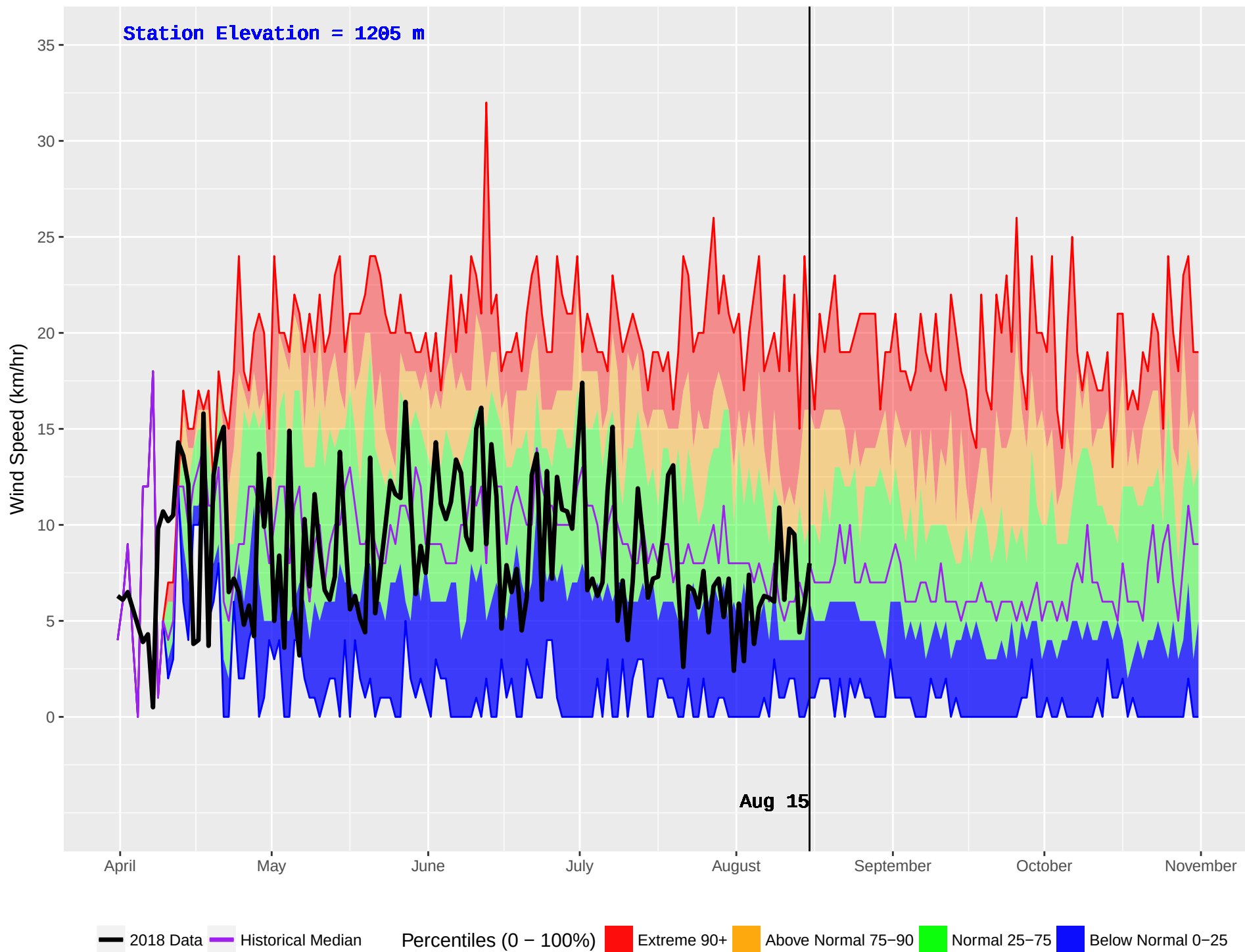
GWYNETH LAKE (309) : Historical (1986–2016) and Current (2018) Daily Wind Speed
