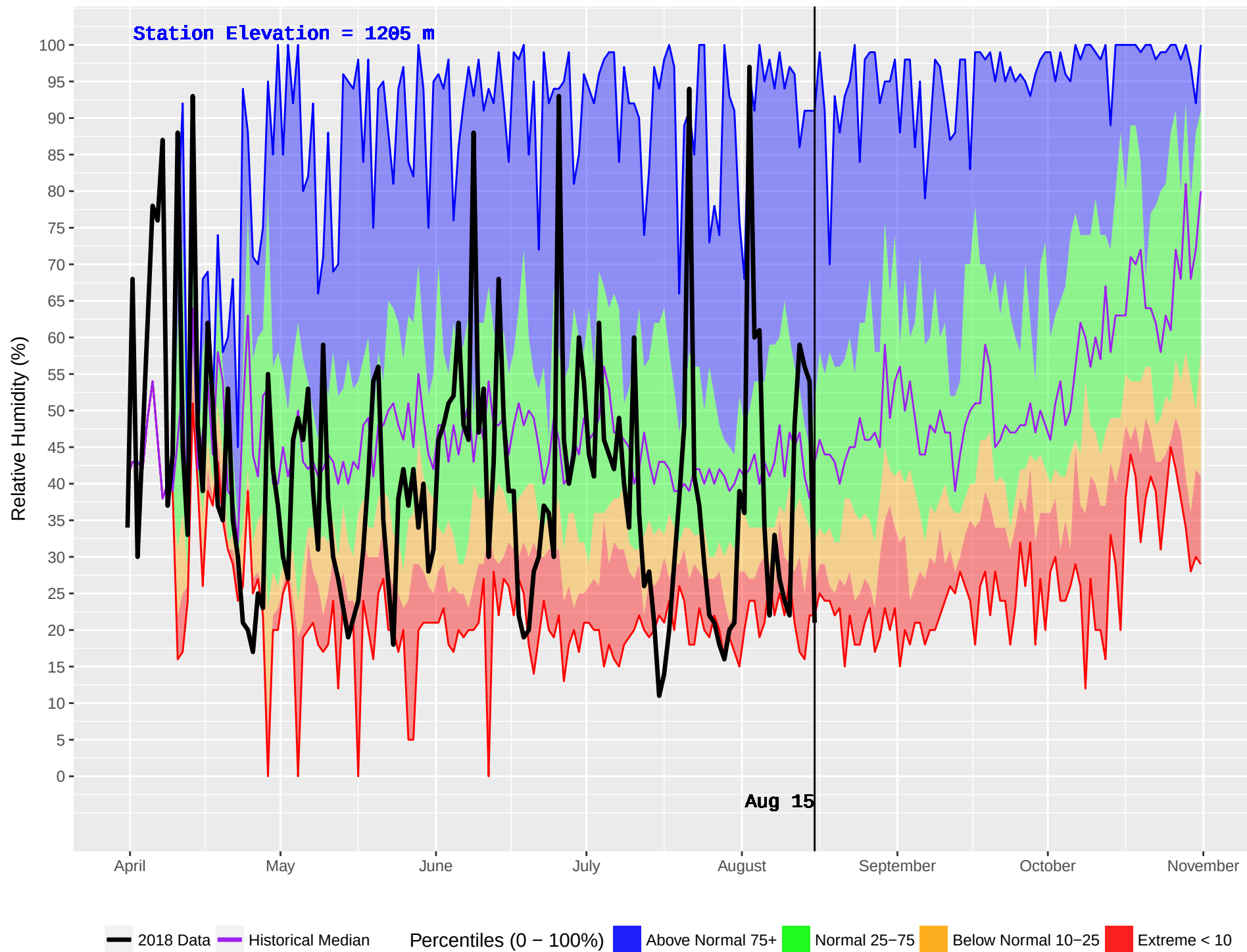
GWYNETH LAKE (309) : Historical (1986–2016) and Current (2018) Daily Relative Humidity
