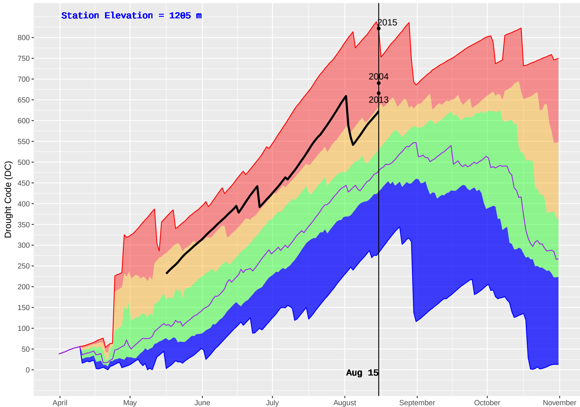
GWYNETH LAKE (309) : Historical (1986–2016) and Current (2018) Daily Drought Code (DC)
