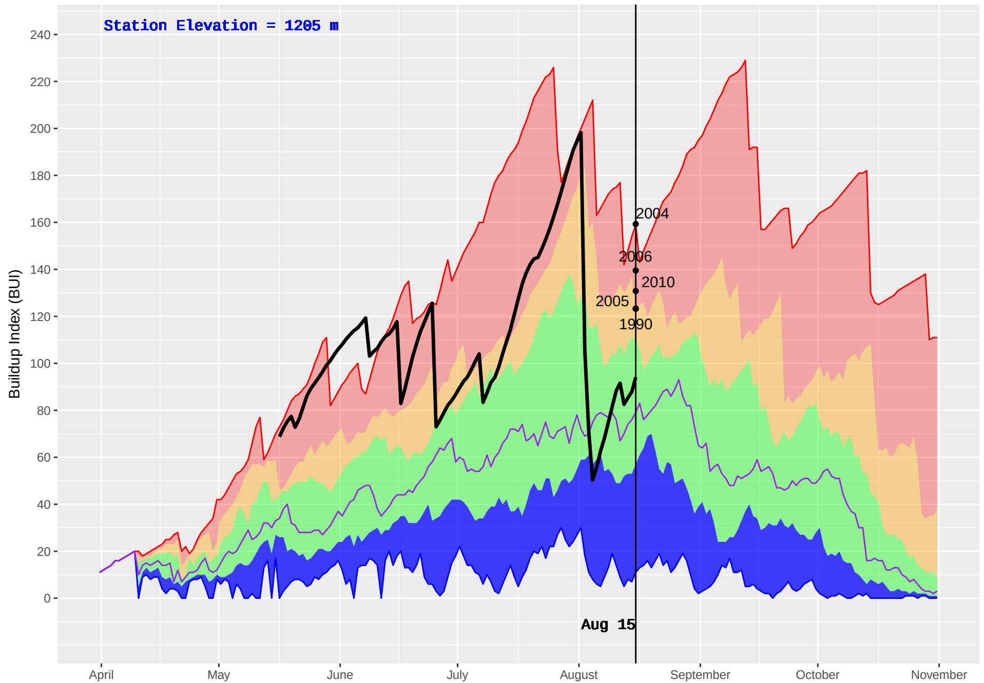
GWYNETH LAKE (309) : Historical (1986–2016) and Current (2018) Daily Buildup Index (BUI)
